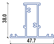
292 DIVISOR
